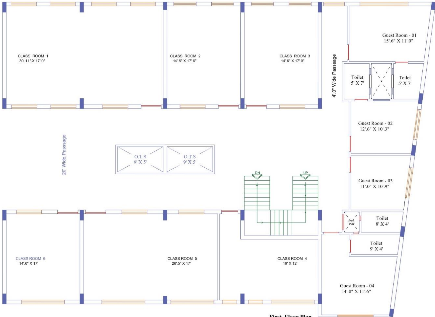
First Floor Plan 4876.00 Sq.Ft
